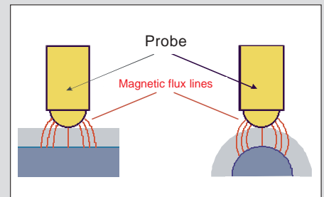
Magnetic flux lines on curved surfaces
